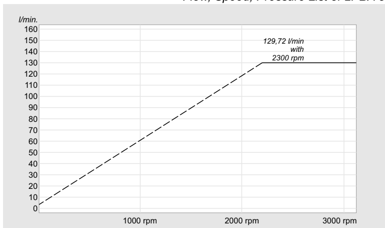
Flow, Speed, Pressure List of 2PBA 56
