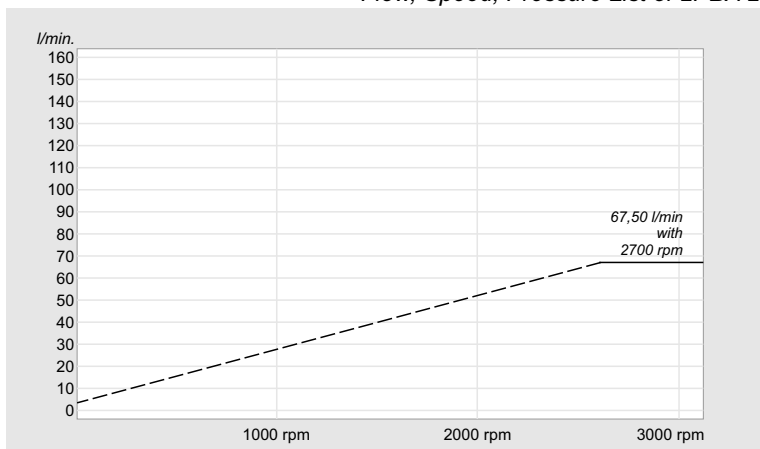
Flow, Speed, Pressure List of 2PBA 25
